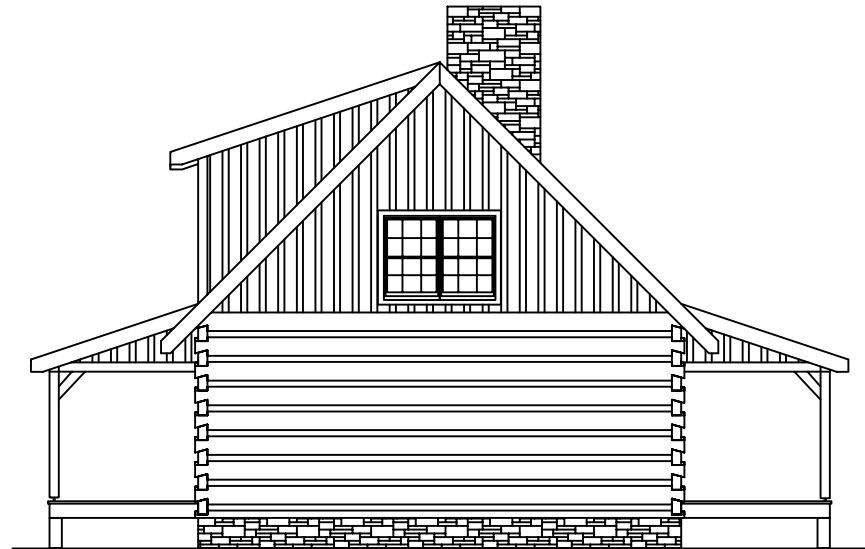
LEFT ELEVATION
