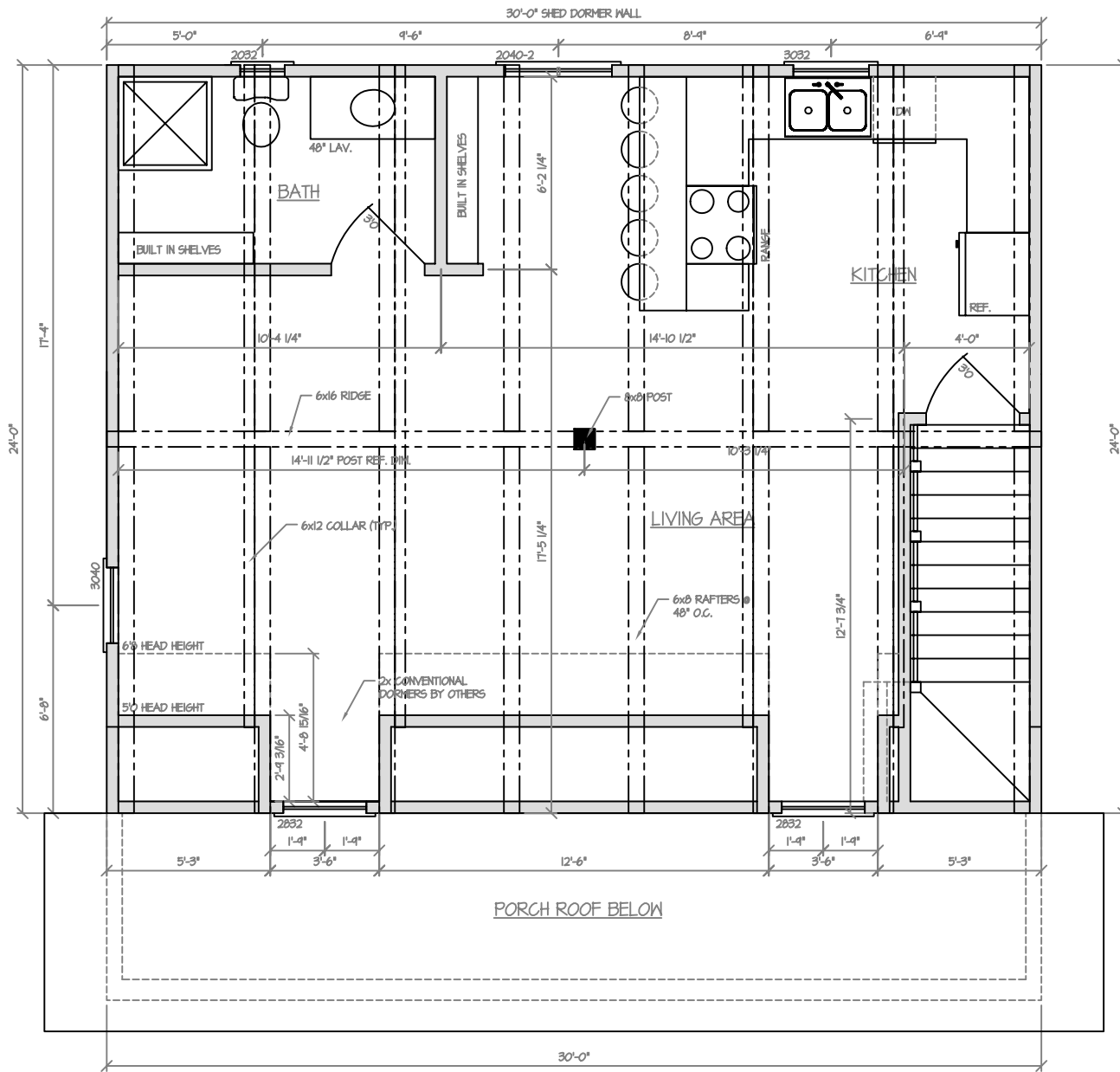
↑ PLAN FRONT SECOND FLOOR GARAGE PLAN
