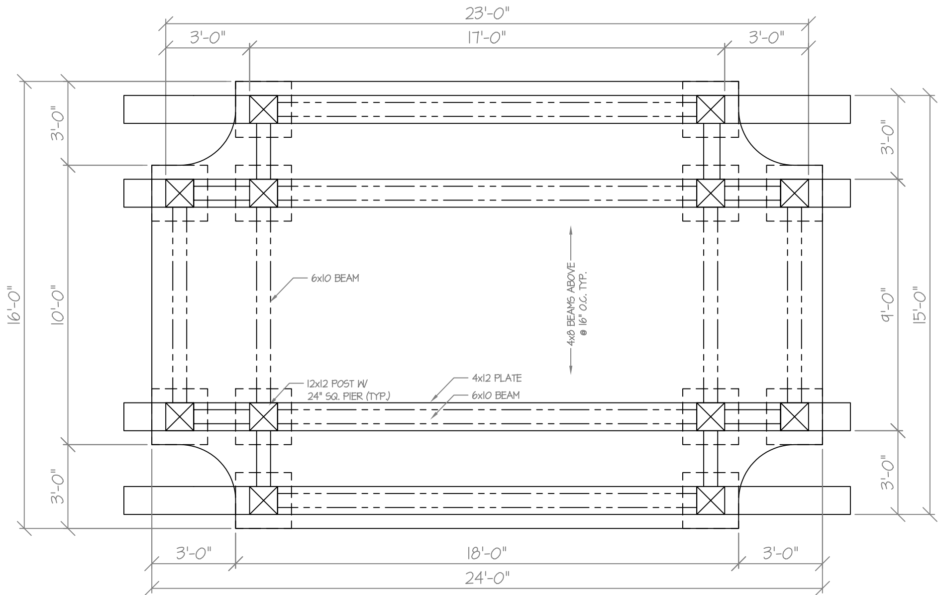
PERGOLA PLAN VIEW
